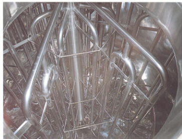
■ Cooled paddle wheel stirrer.
